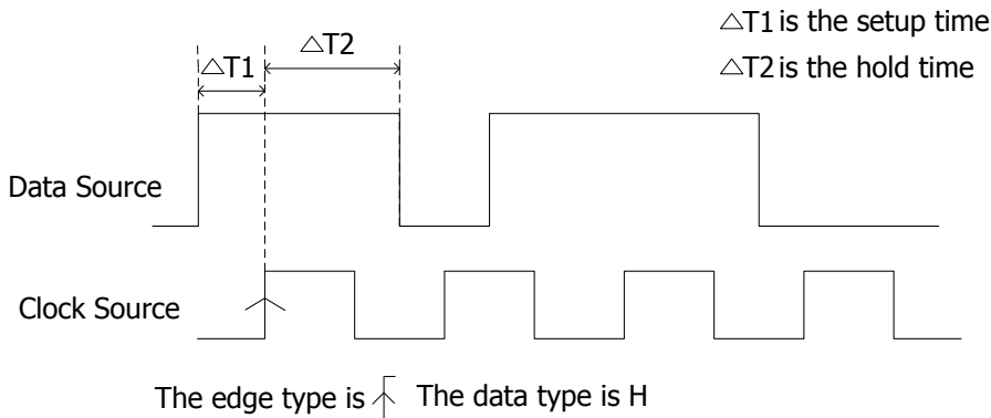
Figure 5-11 Setup/Hold Trigger
