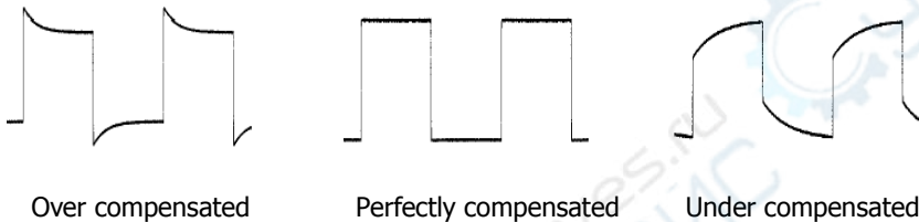
Figure 1-12 Probe Compensation
