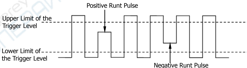
Figure 5-9 Runt Trigger
