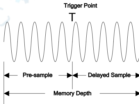
Figure 4-4 Memory Depth
