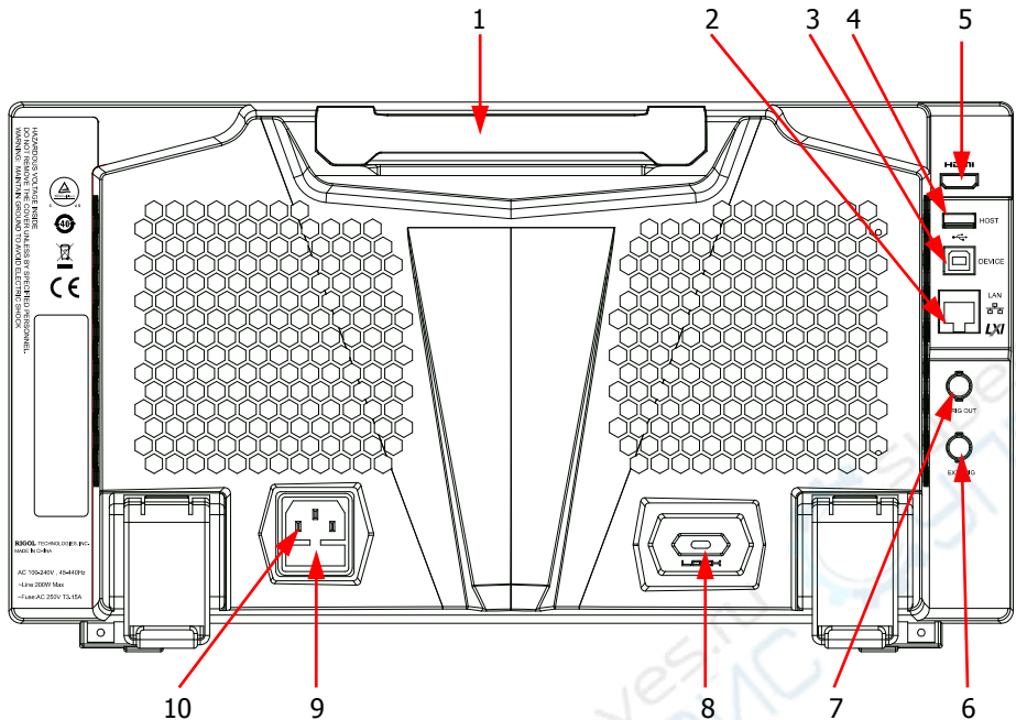
Figure 1-14 Rear Panel
