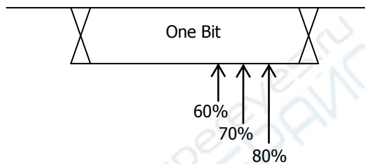
Figure 5-18 Sample Position
